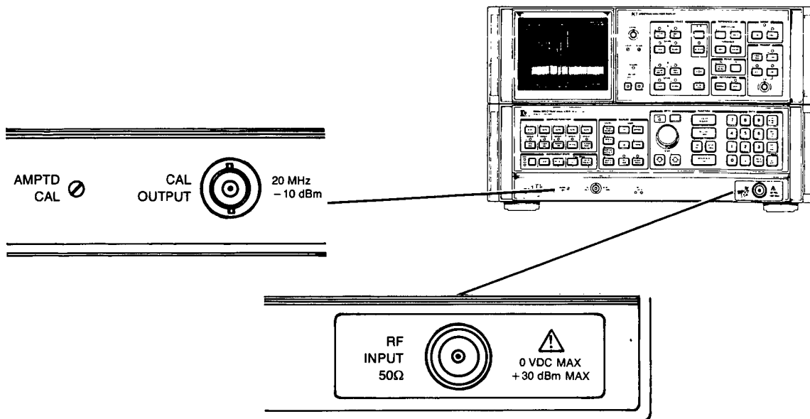
SIGNAL INPUT AND CALIBRATION CONTROLS
